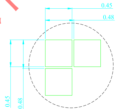
DOTS DETAIL A SCALE 10X
